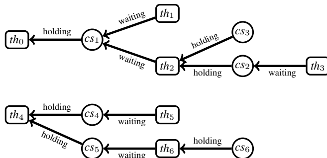
Fig. 2. An instance of a Resource Allocation Graph (RAG).
