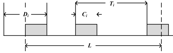
Fig. 3. Densest packing for work-conserving algorithms.
