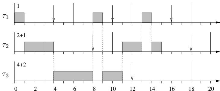
Figure 8.13 Schedule produced by Deadline Monotonic for the task set reported in Table 8.1, when \tau_2 is split in two subjobs of 2 and 1 unit, and \tau_3 is split in two subjobs of 4 and 2 units, respectively.
