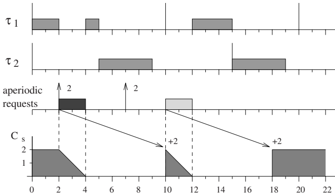
Figure 5.18 Example of a high-priority Sporadic Server.
