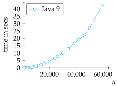
Graph: (a^*)^* \cdot b and strings \underbrace{a \dots a}_n
