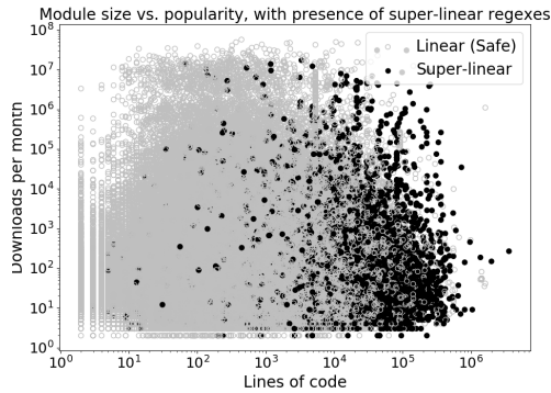
Figure 3: npm modules by size and popularity (log-log). The 13,018 modules with SL regexes are in black.
