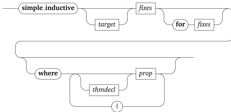
Figure 5.2: A railroad diagram describing the syntax of simple_inductive . The target indicates an optional locale; the fixes are an and -separated list of names for the inductive predicates (they can also contain typing- and syntax annotations); similarly the fixes after for to indicate fixed parameters; prop stands for an introduction rule with an optional theorem declaration ( thmdecl ).
