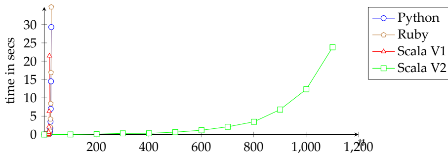
Graph: a^{2\{n\}} \cdot a^{\{n\}} and strings \underbrace{a \dots a}_n
