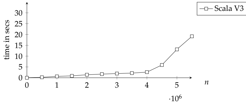
Graph: (a^*)^* \cdot b and strings \underbrace{a \dots a}_n
