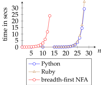
Graph: a^{2\{n\}} \cdot a^{\{n\}} and strings \underbrace{a \dots a}_n
