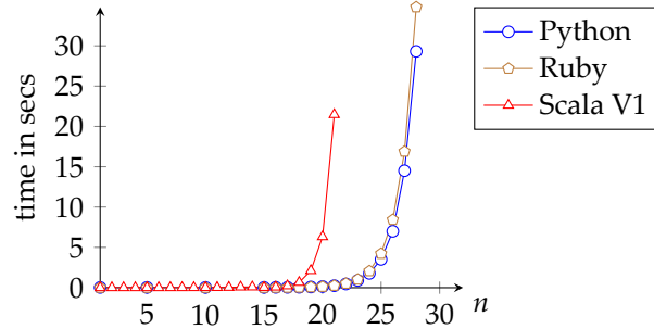
Graph: a^{2\{n\}} \cdot a^{\{n\}} and strings \underbrace{a \dots a}_n
