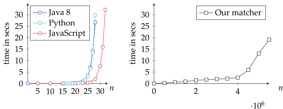
Graphs: (a^*) \cdot b and strings a . . . a n
