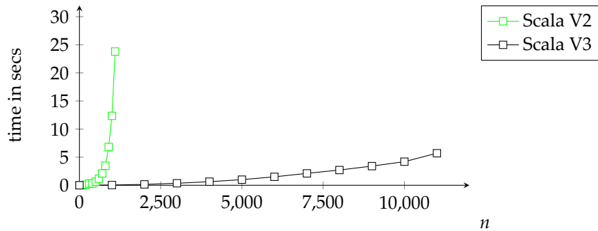
Graph: a^{?{n}} \cdot a^{n} and strings \underbrace{a \dots a}_n
