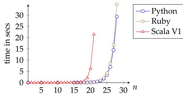
Graph: a^?{n} \cdot a^{n} and strings \underbrace{a \dots a}_n
