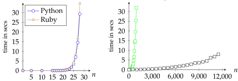
Plots: a^?{n} \cdot a^{n} and strings \underbrace{a \dots a}_n
