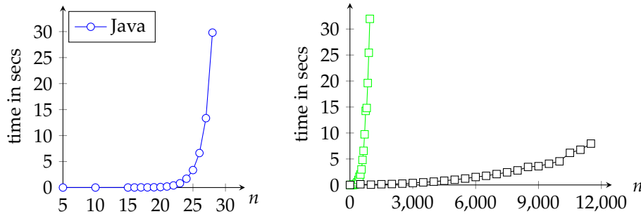
Plots: (a^*)^* \cdot b and strings \underbrace{a \dots a}_n
