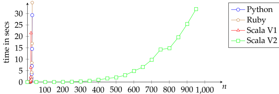
Plot: a^{2\{n\}} \cdot a^{\{n\}} and strings \underbrace{a \dots a}_n
