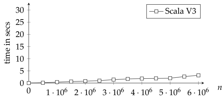
Plot: (a^*)^* \cdot b and strings \underbrace{a \dots a}_n
